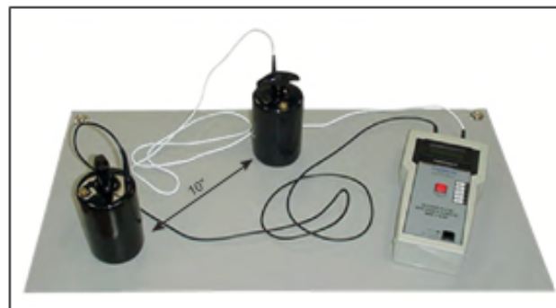
Figure 4. Setting up for Rtt testing.
