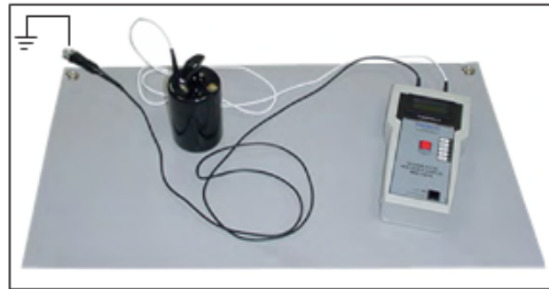
Figure 3. Setting up for RTG testing.
